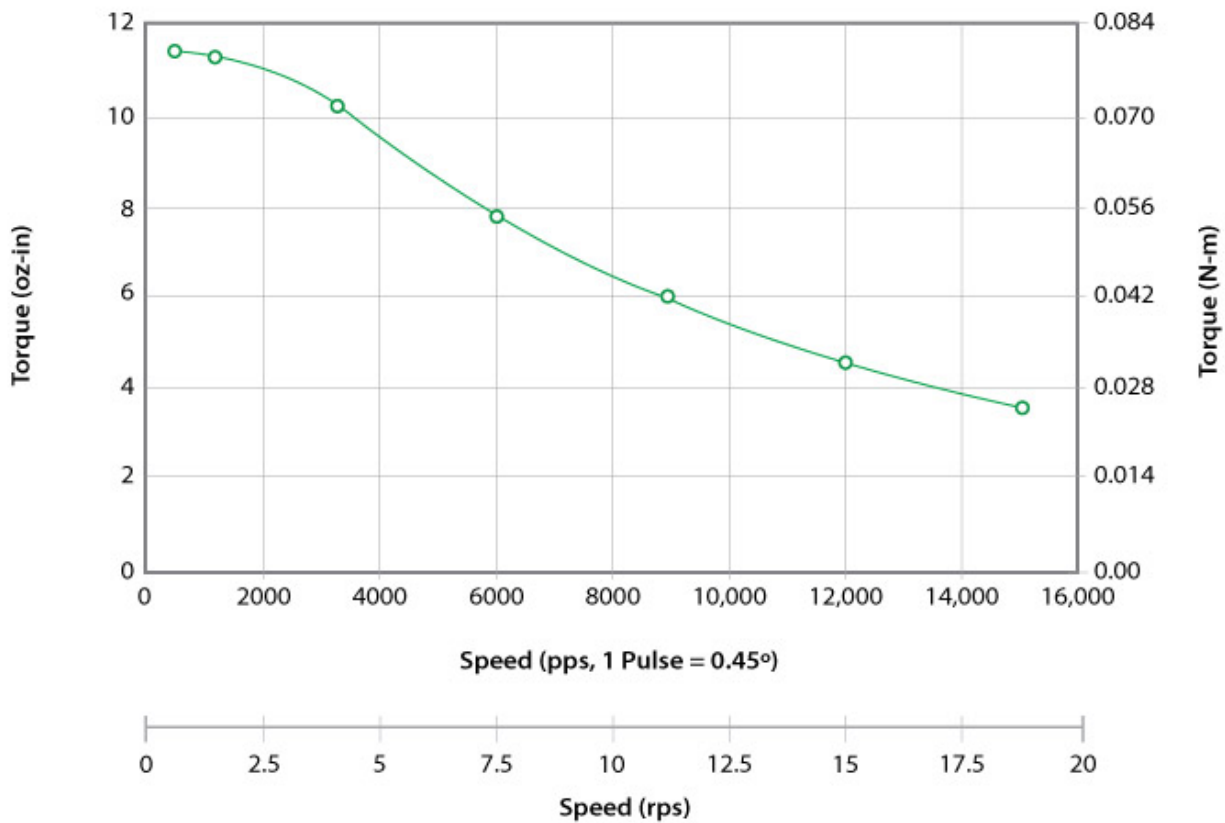
ZN417-11-18 (0.9° Step Motor) 24VDC, 0.84 Amp Peak, Bipolar, 1/2 Stepping
